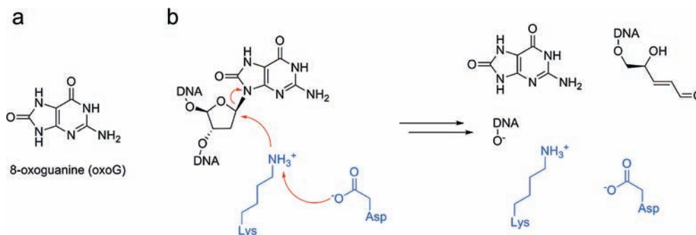
Figure 1. DNA glycosylase substrate and mechanism. (a) Chemical structure of 8-oxoguanine (oxoG), generated by oxidative damage of DNA by reactive oxygen species. (b) Overview of Schiff-base enzymatic mechanism of DNA glycosylases responsible for excision of oxoG from oxidatively damaged DNA. An Asp side chain is proposed to deprotonate a nearby Lys side chain, which proceeds to undergo a nucleophilic attack on the C1' atom of the oxoG nucleotide, ultimately leading to strand cleavage at the 3' phosphate group.
